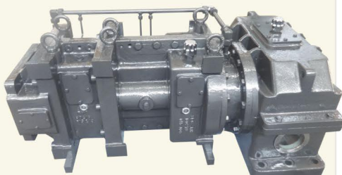
Counter Rotating Twin Screw Extruder Gearbox
